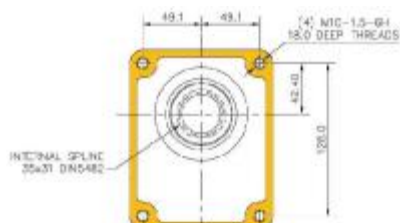
Group 3P Pump Flange
