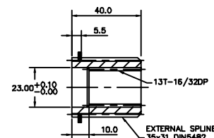
13T-16/32DP Spline Bore
