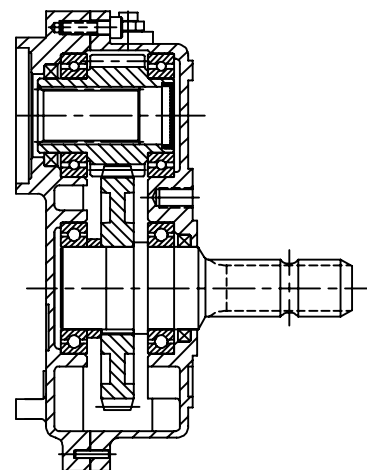
Male Input Shaft
