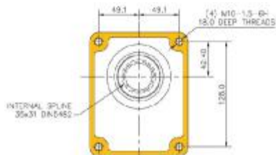
Group 3P Pump Flange
