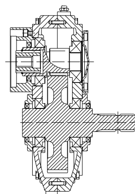
Male Input Shaft
