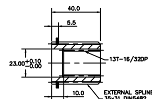
13T-16/32DP Spline Bore
