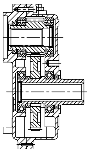
Female Input Shaft
