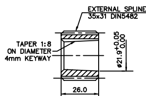
4mm Tapered Keyed Bore
